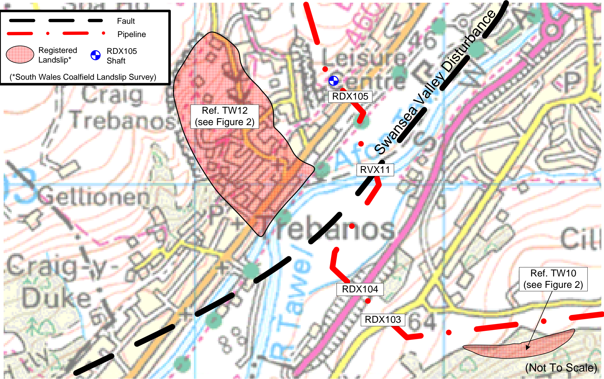
FIGURE 1: TREBANOS GEOLOGICAL LANDSLIP AND FAULT DATA
